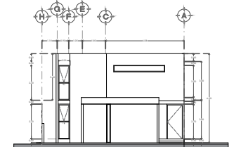
FACHADA PRINCIPAL ESC: 1:100
